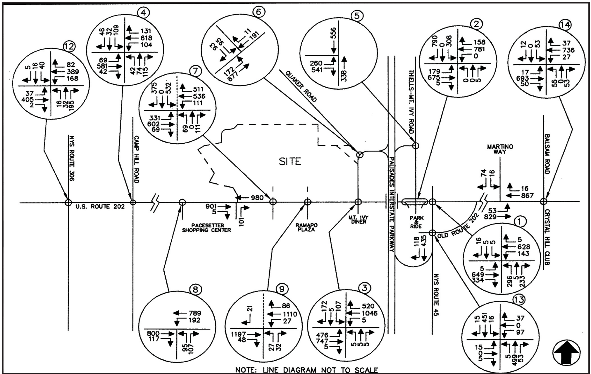
Figure 3.5-35: 2011 Build Traffic Volumes Weekend Peak Saturday Highway Hour (With Patrick Farm) Minisceongo Park Towns of Haverstraw & Ramapo, Rockland County, New York Source: John Collins Engineers, P.C. Date: October, 2008
